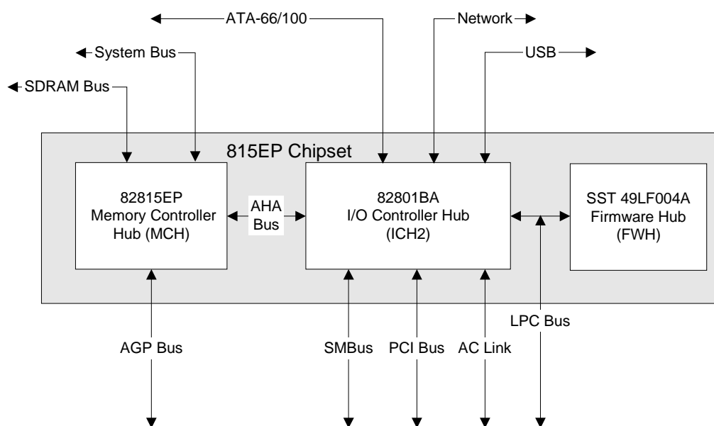
Figure 7. Intel 815EP Chipset Block Diagram
